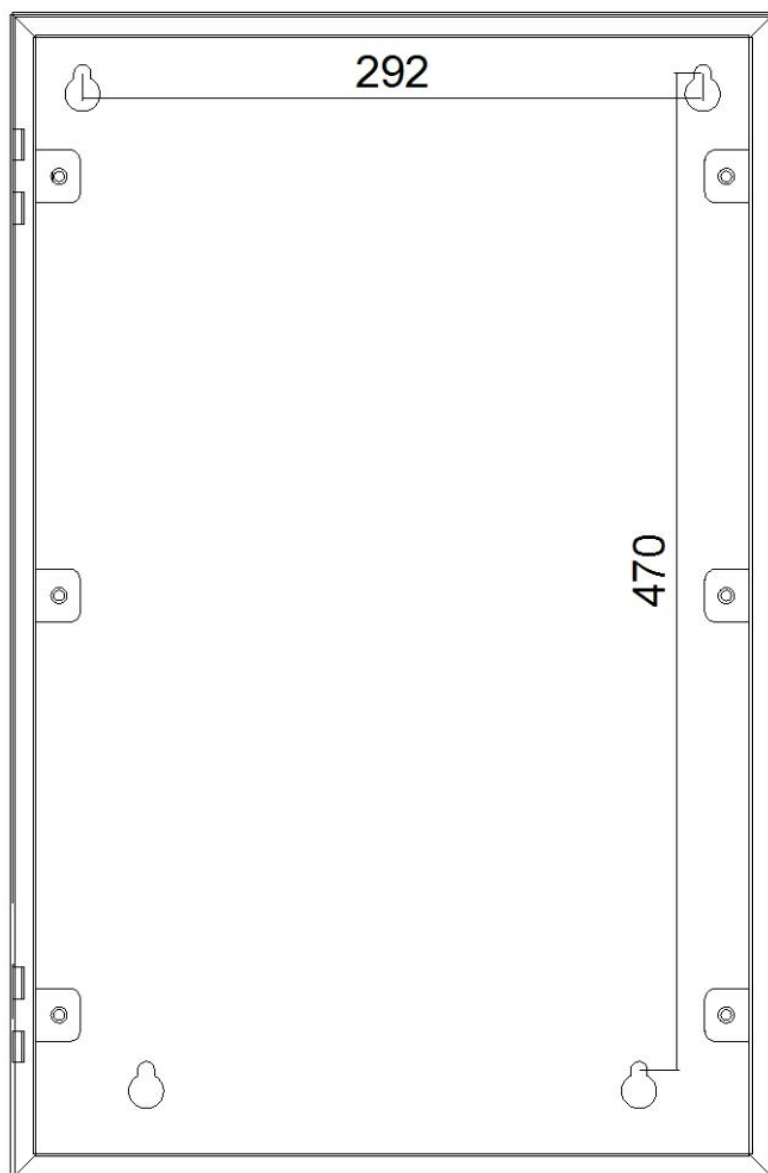
Mounting details
