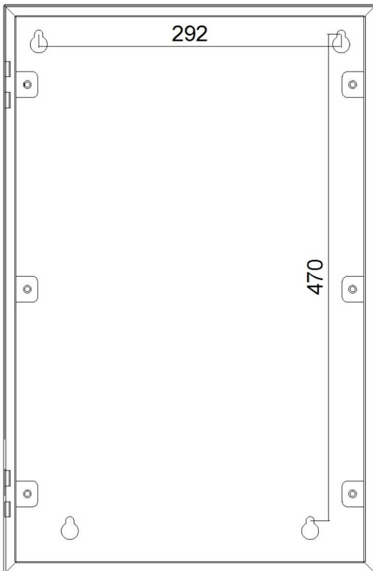
Mounting details
